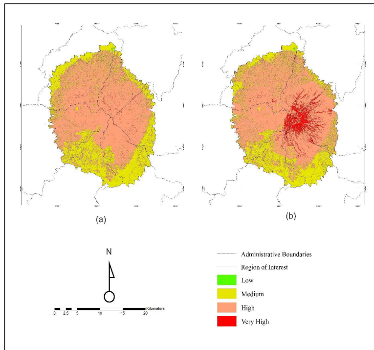
Fig. 4 Landslide Hazard Map (a) August 2016 (b) April 2017
