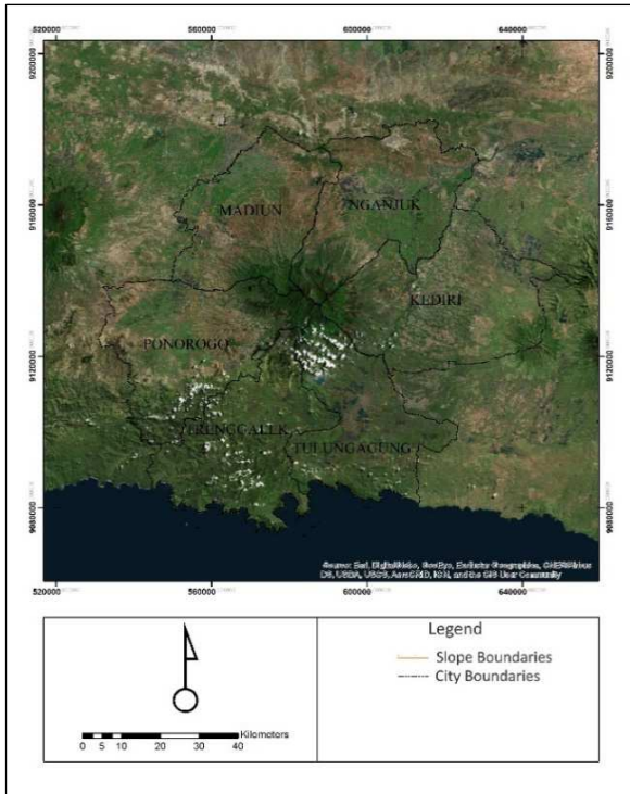
Fig. 1 Location of Mount Wilis
