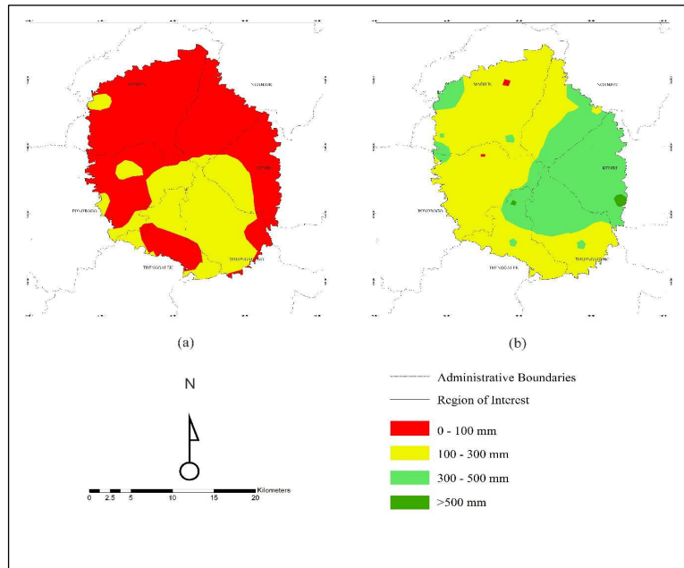
Fig. 3 Rainfall Distribution Map (a) July 2016 (b) March 2017
