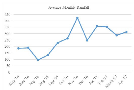
Fig. 2 Monthly rainfall from rain gauge
