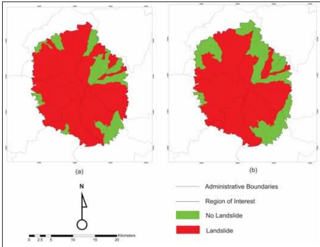
Fig. 5 Landslide events in (a) 2016 (b) 2017
